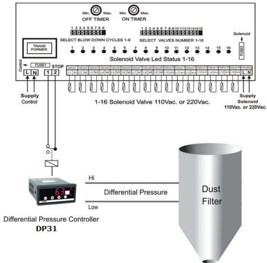
Example of connection with Jet Pulse JP16.
